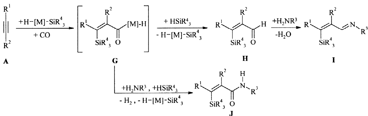
Scheme 3. Formation of 4-silylated azadienes from alkynes by silylformylation in the presence of amines
