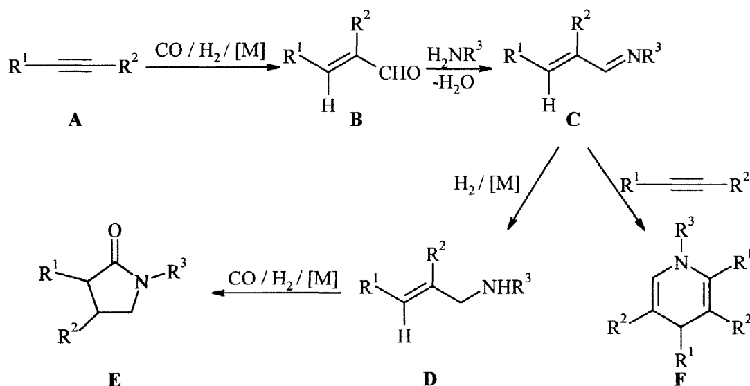
Scheme 1. Carbonylation of alkynes in the presence of primary amines
