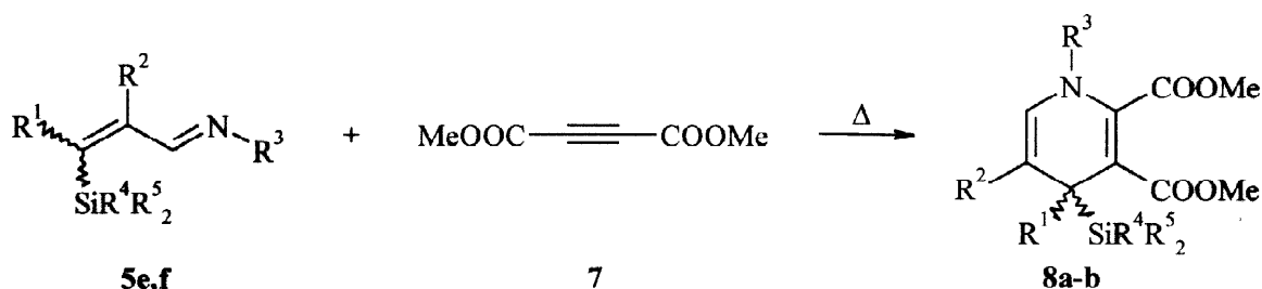
Scheme 5. Diels-Alder reaction of azadienes 5 with dimethyl acetylene dicarboxylate 7
