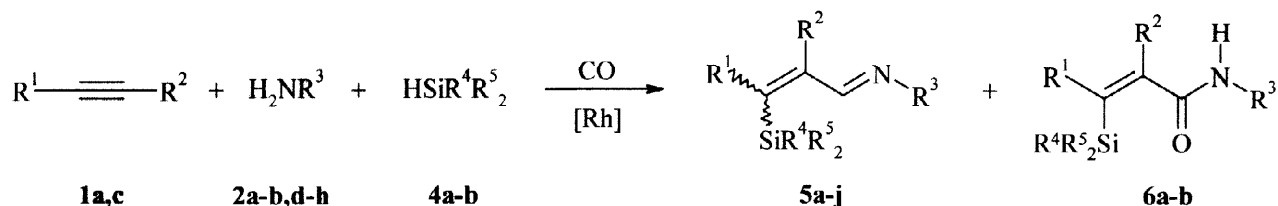
Scheme 4. Silylformylation of alkynes in the presence of primary amines
