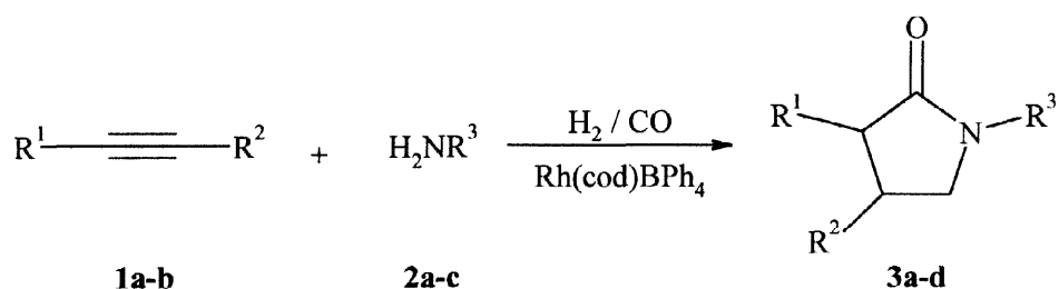
Scheme 2. Synthesis of 2-pyrrolidinones via hydrocarbonylation of alkynes in the presence of primary amines
